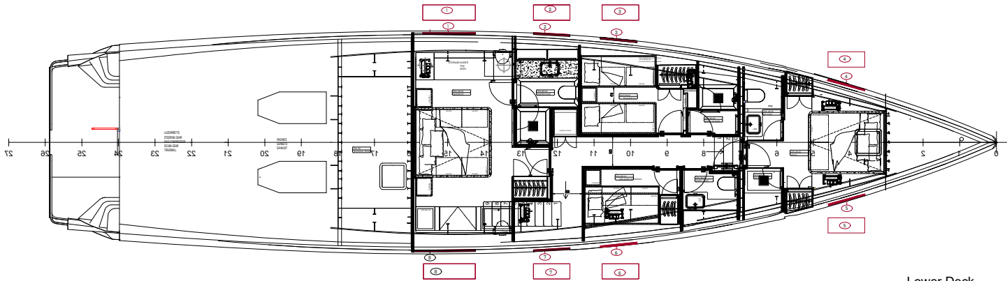
Lower Deck
